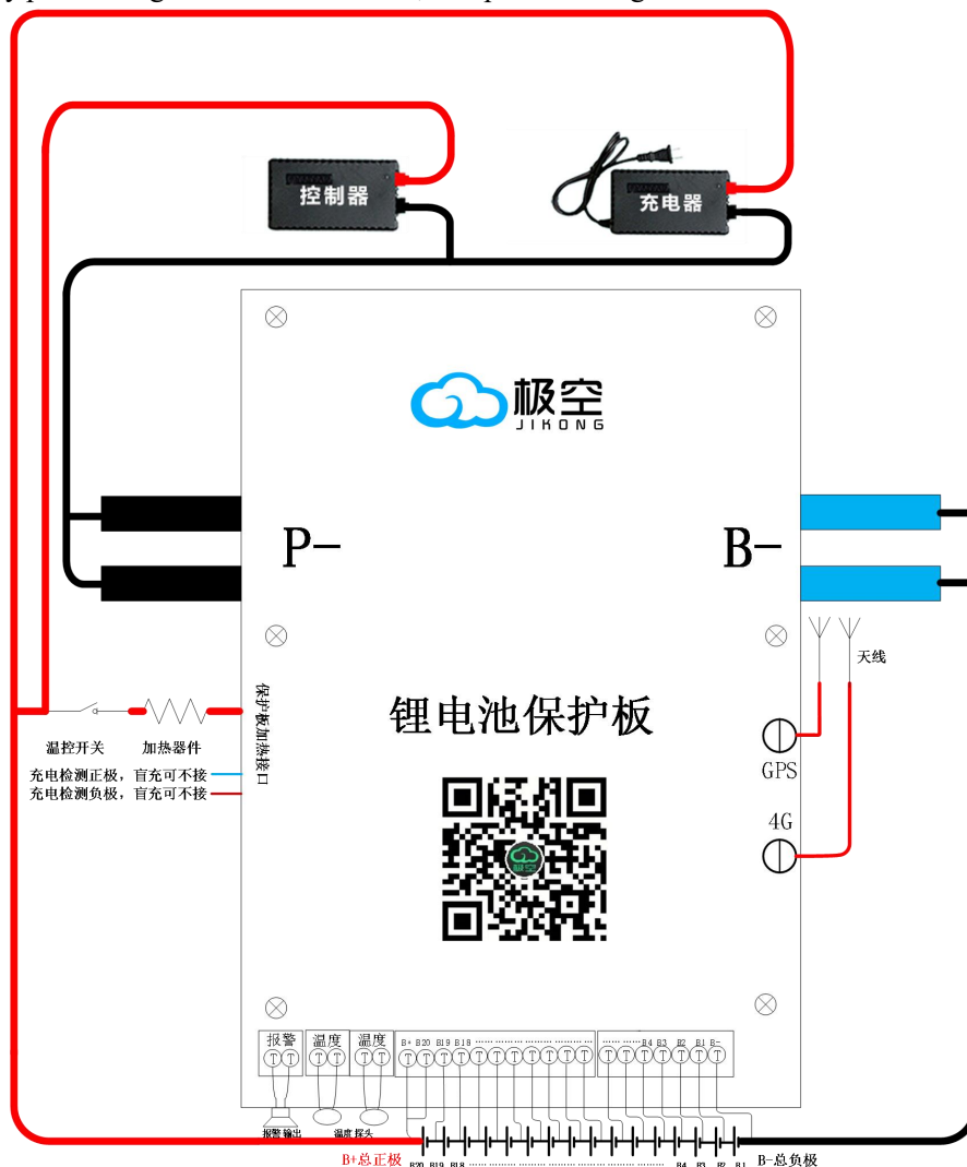
JK-BD4AxxS-6PRG接线图
